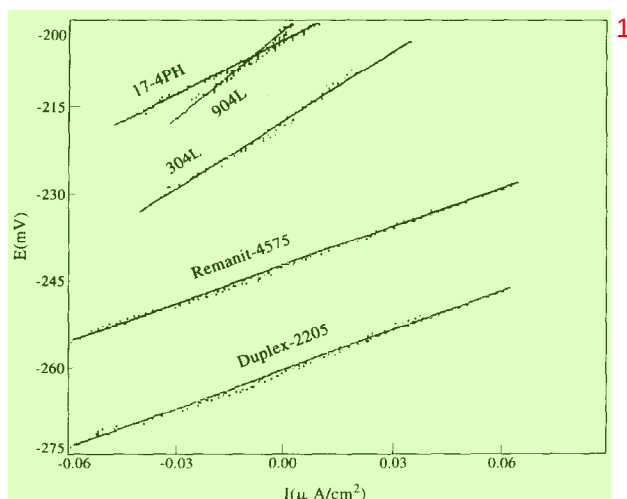
Fig. 1. Typical polarization resistance curves for different types of stainless steels in seawater at 50°C.
