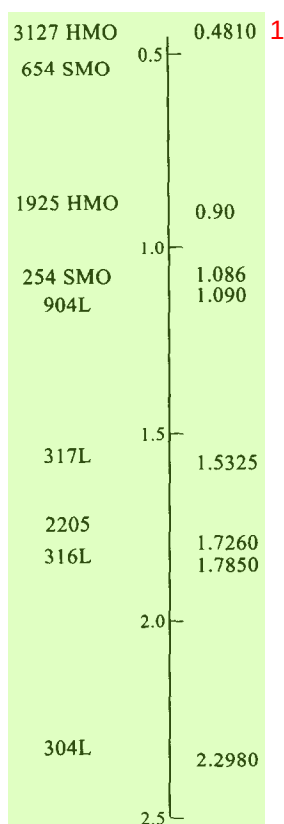
Fig. 4. Predicted ranking of conventional and high alloy stainless steels. 2
