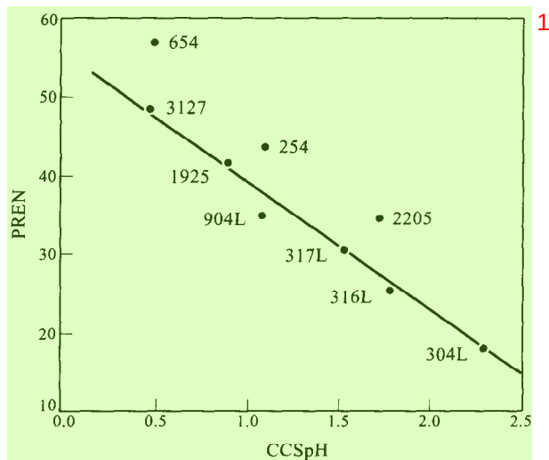
Fig. 7. Plot of PREN vs CCSpH for steel in natural seawater and NaCl solution.
