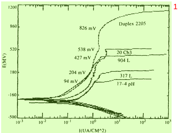
Fig. 2. Potentiodynamic polarization plots for different steels in seawater at 50°C.
